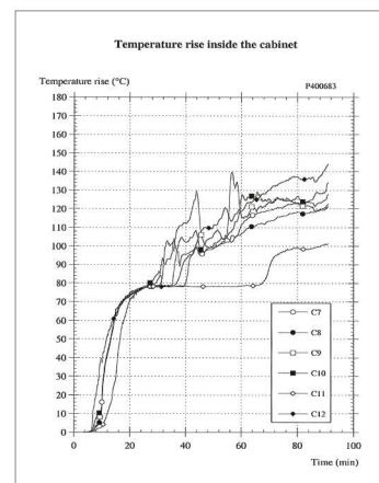
● Heat Graph (C7-12)
