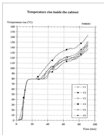
● Heat Graph (C1-6)
